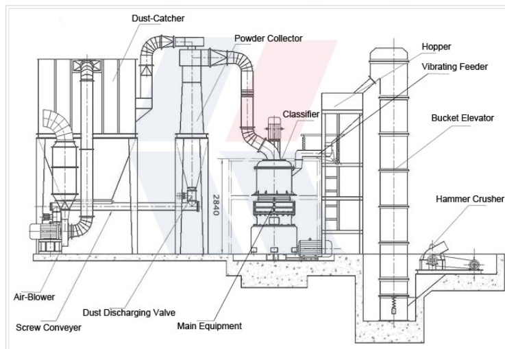
CZM80 Three-ring Micro Powder Mill Diagram of the Equipment
